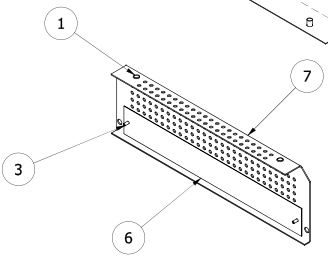
X2 FOR ASSEMBLY AC-61818
