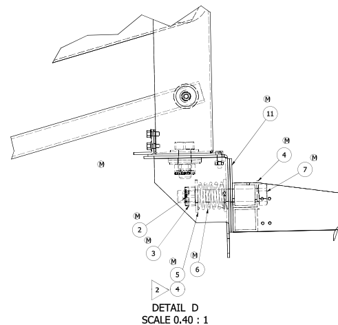
DETAIL OF PYROMETER BOX
